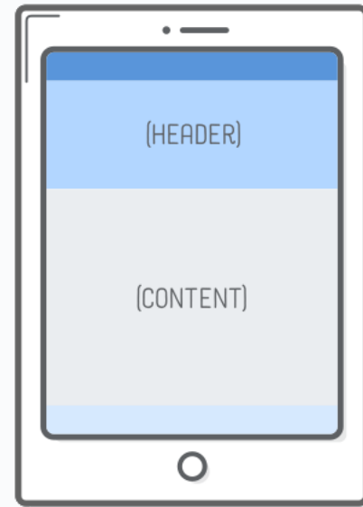
ZOOM DISABLED
