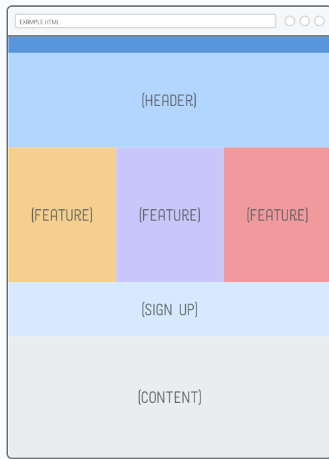
AFTER REORDERING
