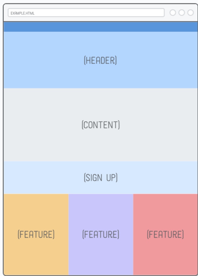
BEFORE REORDERING
